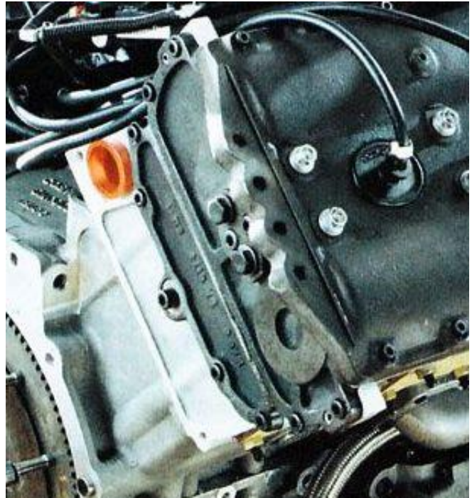
Lead wire in place
